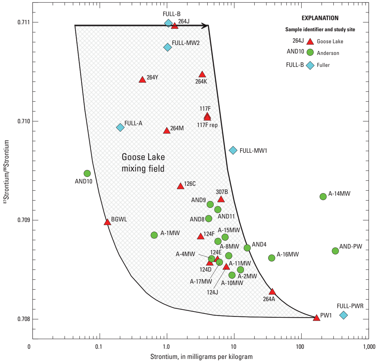
Figure B-4. Strontium (Sr) concentration compared to 87 Sr/ 86 Sr values for water samples from all three study sites: Goose Lake, Anderson, and Fuller.
